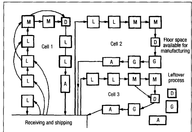
Figure 2 Three-Cell Manufacturing System (Black 1991)
