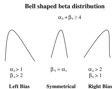
Fig. 2. Shapes of the beta distribution that ensures a bell-shaped beta distribution.
