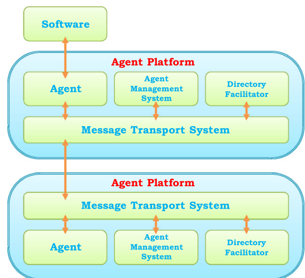
Fig. 2. Agent management reference model (Bellifemine et al., 2001).
