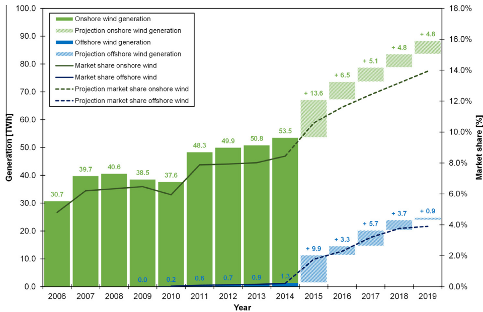
Fig. 1. Increasing importance of wind energy in the German electricity market [4–6].
