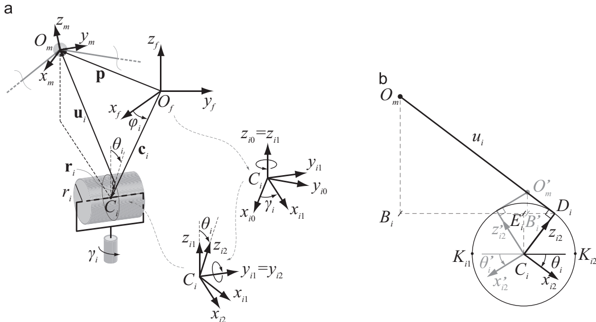
Fig. 2. Sketch of the cable-driven system. (a) Main reference systems and (b) plane of the i th pulley.
