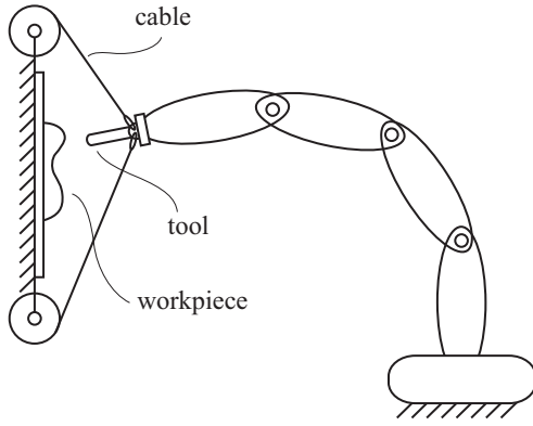
Fig. 1. Concept of the static performance improvement.
