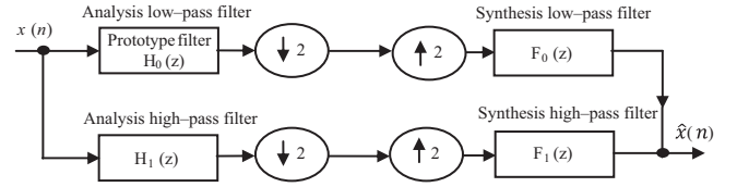
Fig. 1. The 2-channel quadrature mirror filter bank.
