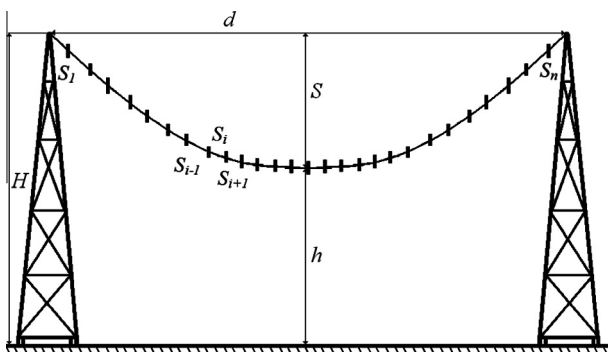
Fig. 1. Line dimensions of the catenary.
