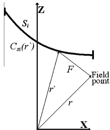
Fig. 2. Presentation of segment S_i and field point.
