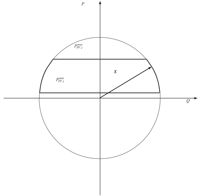
Fig. 1. Loading capability chart of the i -th photovoltaic generator.
