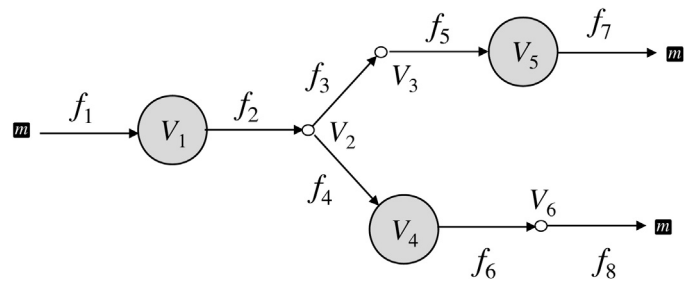
Fig. 1. Distribution system with N=6 nodes and M=8 pipes.
