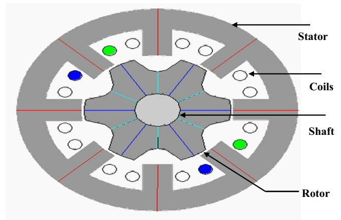
Fig. 2. The SRM 8/6 poles construction.
