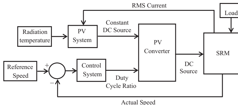
Fig. 1. The overall system for SRM control.
