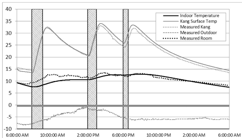
Fig. 1. Predicted and measured temperature profile on 2/19/2009.
