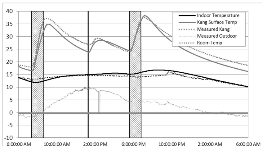
Fig. 2. Predicted and measured temperature profile on 11/24/2008.
