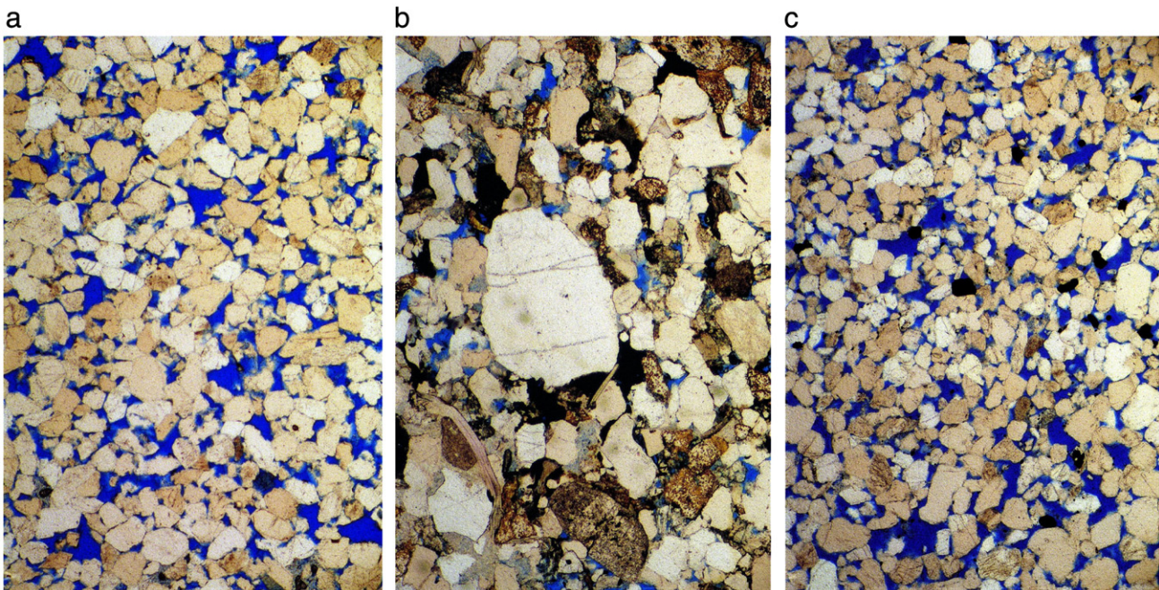
Fig. 1. Thin section photomicrographs. a) Sandstone from Craigeith Quarry in Edinburgh, typical of the stone used during the late 18th and 19th centuries as ashlar block in Edinburgh New Town. The Craigeith sandstone is no longer available as the quarry is closed and infilled. b) Sandstone from a quarry in Derbyshire currently used for stone repairs in Edinburgh New Town. c) Sandstone from Cullaloo Quarry, Fife, north of Edinburgh which has similar petrographic characteristics to Craigeith sandstone. This quarry has recently been reopened to supply stone for the conservation and repair of historic buildings in Edinburgh. Images are 4 mm high.
