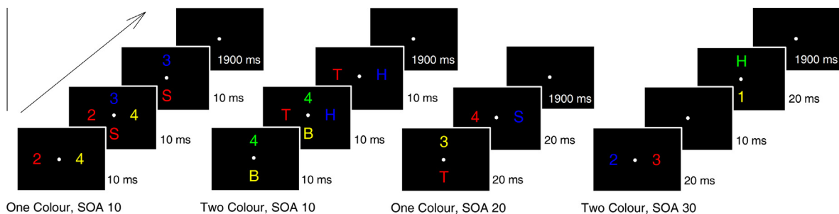
Fig. 1. Stimulus procedures. Schematic illustration of the time course of stimulus events in our previous ERP experiments (Eimer & Grubert, 2014; Grubert & Eimer, in press ) and in the current behavioural study. On each trial, two displays with a colour-defined target and a nontarget-colour distractor on opposite sides were presented sequentially. One target/nontarget pair appeared on the horizontal meridian and the other on the vertical meridian. In the One Colour task, all targets had the same colour. In the Two Colour task, there were two possible target colours, and target colour always changed between the first and second display. Each display was presented for 20 ms, and the SOA between the two displays was either 10 ms, 20 ms, or 30 ms. In SOA10 trials, the second display appeared 10 ms after the onset of the first display, so that both displays were simultaneously present for 10 ms. In SOA20 trials, the onset of the second display was synchronous with the offset of the first display. In SOA30 trials, there was a 10 ms gap between the offset of the first and the onset of the second display. The examples shown in this figure include One Colour trials where both targets are red and Two Colour trials where the two targets are red and green, and all three SOA conditions. In our earlier ERP studies, participants had to judge the alphanumeric category of the two target objects (same/different). In the current study, their task was to report whether the first target-colour item on each trial was a letter or a digit. (For interpretation of the references to colour in this figure legend, the reader is referred to the web version of this article.)
