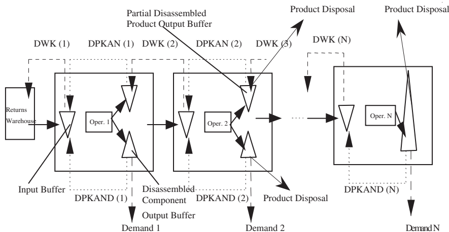
Fig. 1. Multi Kanban system for disassembly.
