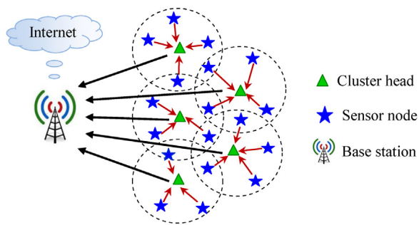
Fig. 1. A wireless sensor network model.
