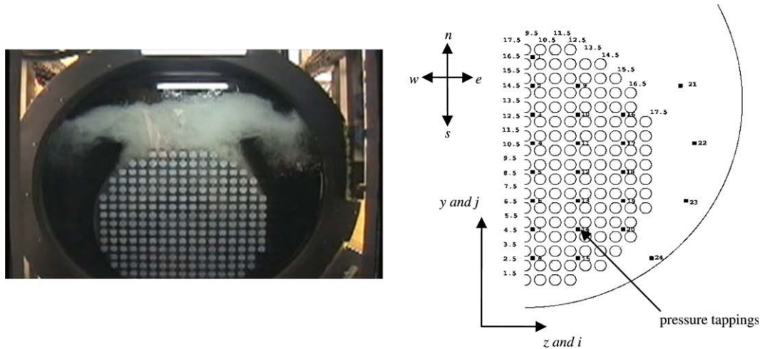
Fig. 1. Front view and tube layout of a kettle reboiler.
