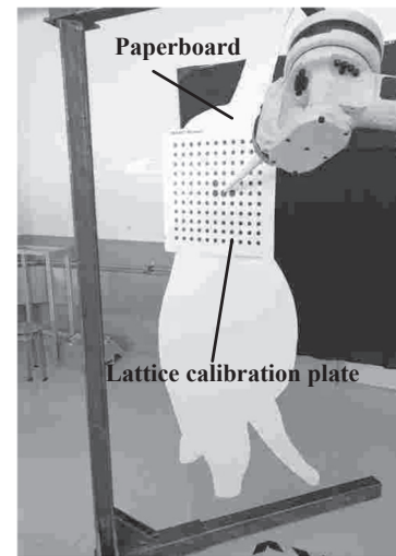
Fig. 3. User coordinate system calibration.
