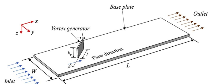
Fig. 1. Schematic diagram of the considered rectangular vortex generator fixed over a baseplate.
