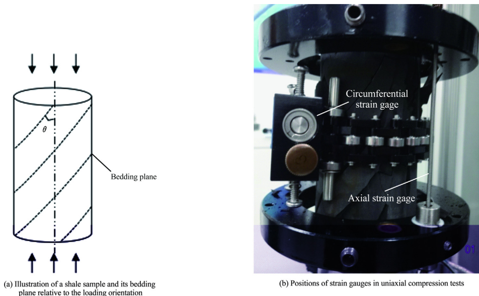
Fig. 1. Illustration of shale sample and testing apparatus.
