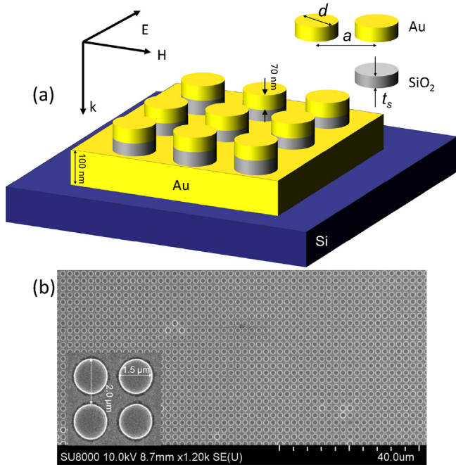
Fig. 1. (a) The schematic drawing of a disk-shaped MMA consisting of a SiO 2 layer sandwiched by a 70 nm Au pattern on top of 100 nm Au film. The whole structure is formed on the surface of a Si substrate after the deposition of a 5-nm Cr adhesion layer (not shown here). (b) A SEM image of a typical sample with a disk diameter d of 1.5 and a periodicity a of 2.0 \mu\text{m} .
