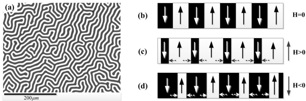
Fig. 1. (a) Magnetic domain pattern of the magneto-optical garnet film, imaged by Faraday microscopy in a polarizing microscopy; Lateral schematic of domains (b) without magnetic field; (c) with an upward magnetic field; (d) with a downward magnetic field.
