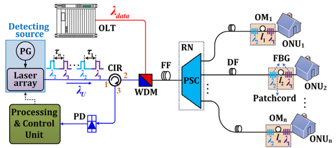
Fig. 1. Principle of the self-match based on polling scheme in a PON.
