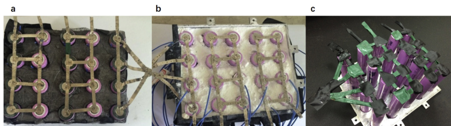
Fig. 1. Photographs of the Li-ion battery packs with different PCMs: (a) the 60 wt% RT44HC/EG composite; (b) the 60 wt% RT44HC/fumed silica composite; (c) no PCM.
