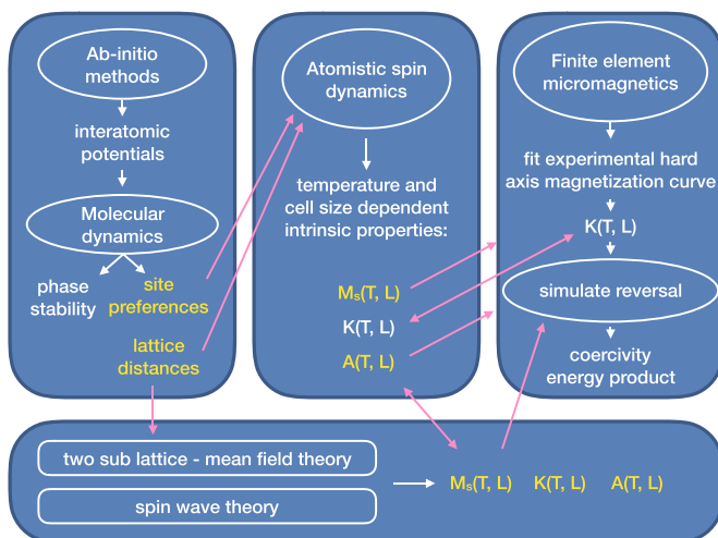
Fig. 1. Schematic of the multiscale process for magnetic materials. The arrows indicate the interactions between the various computational and analytical approaches and show the paths taken for the exchange of information between the model lengthscales. While the mean field and spin wave theories are beyond the scope of this review they are included for completeness, showing their important role in verification of numerical approaches.
