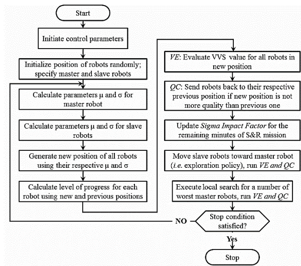
Flow chart of the proposed SRSR optimization algorithm
