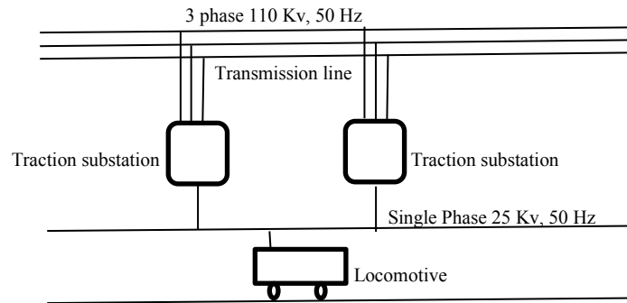
Fig. 1 Traction systems
