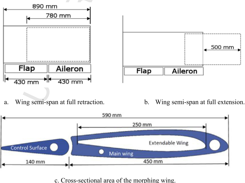
Fig. 2. Final control surface configuration concept.
