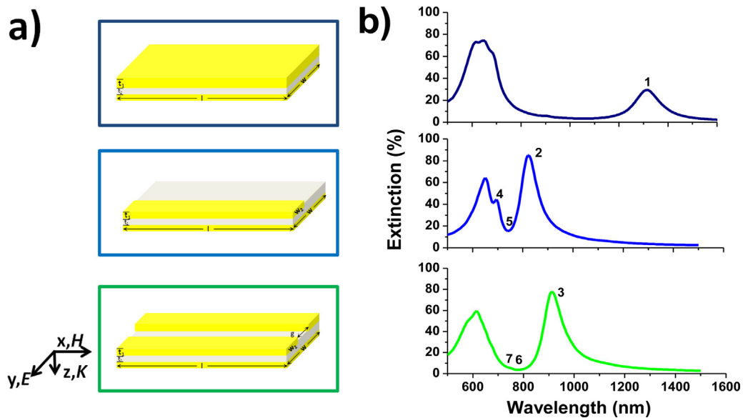
Fig. 1. a) 3D sketches of MIM nanorod, A-MIM nanorod, and MIM nanorod dimer from top down. b) Extinction spectra of the shown nanostructures.
