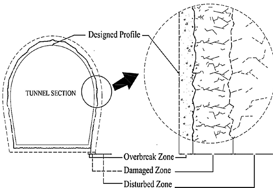
Fig. 1. Blast induced Rock Mass Damage Zone Tunnels (Adapted from Singh and Xavier, 2005).
