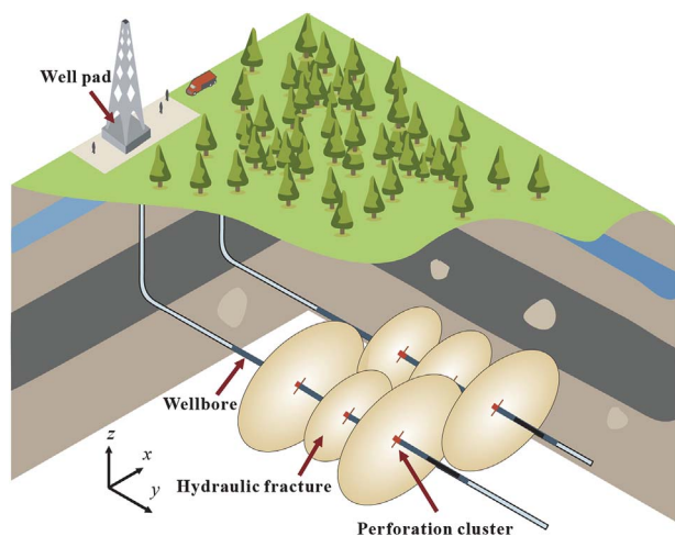
Fig. 1. A diagram of multi-well fracturing at two parallel horizontal wells. Multiple hydraulic fractures are simultaneously or alternately propagating at two wells.
