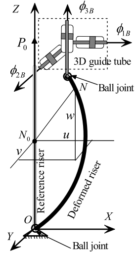
Fig. 1. Riser coordinates and boundary conditions.
