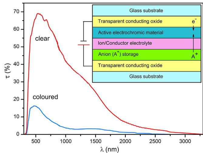
Fig. 1. Optical transmittance spectra of the EC device in the full bleaching (red line) and full colouring (blue line) states. In the insert the multilayer structure of the EC device is shown. (For interpretation of the references to colour in this figure legend, the reader is referred to the web version of this article.)
