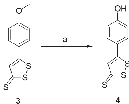
Scheme 1. Reagents and conditions: (a) pyridine hydrochloride, 220 °C.
