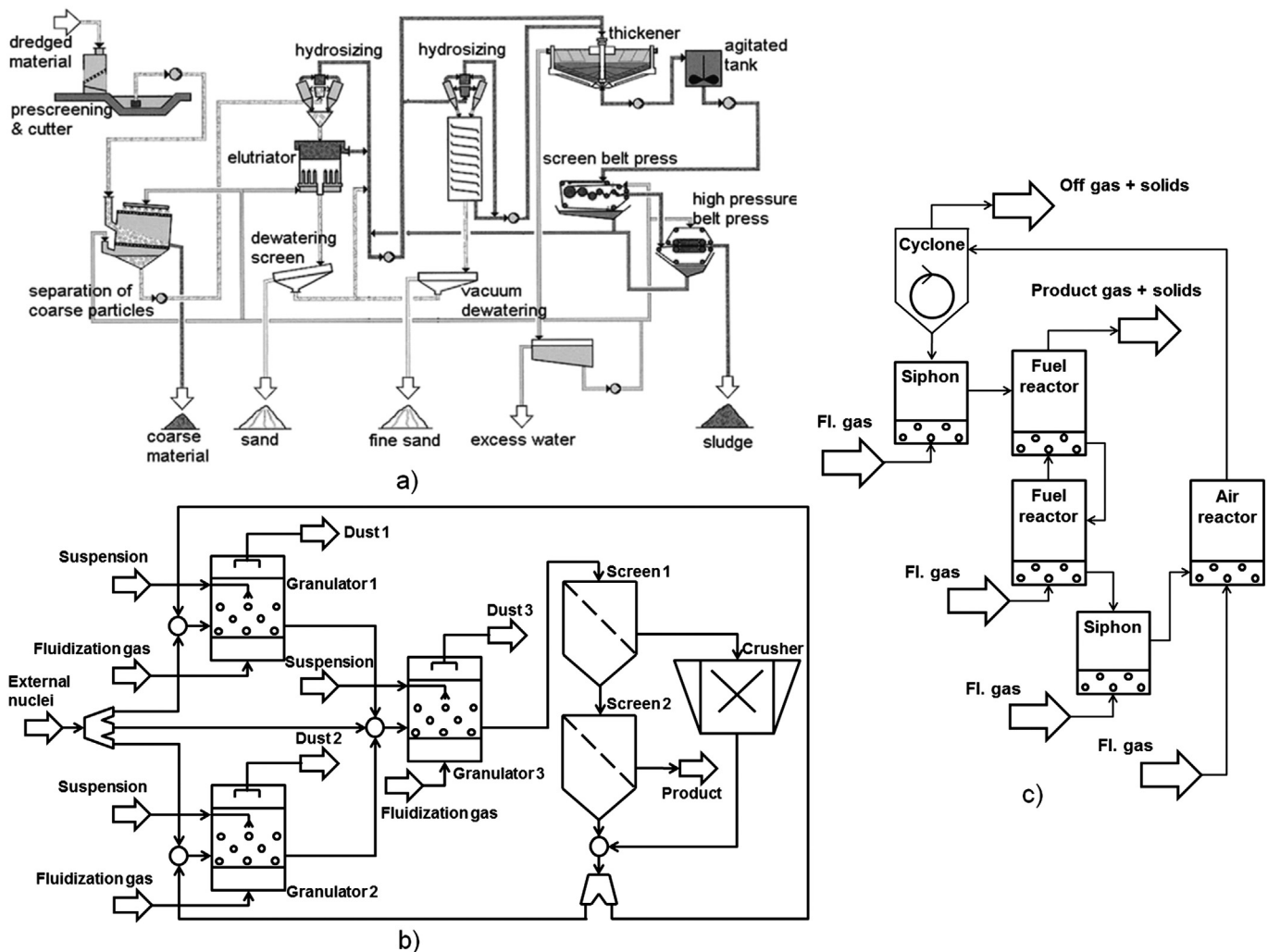
Fig. 1. Examples of solids production processes: soil dewatering and separation [4] (a); granulation (b); chemical looping combustion (c).
