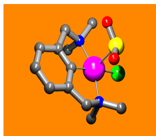
1986, NCN-PtBr(\eta^1-SO_2)
