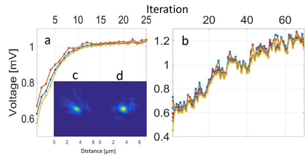
Fig. 2. Second harmonic signal of 800 nm light (a) and 2 \mu m light (b) generational improvement charts. Focal spot images are taken for deformable mirror shape before (c) and after (d) correction for the 800 nm case.
